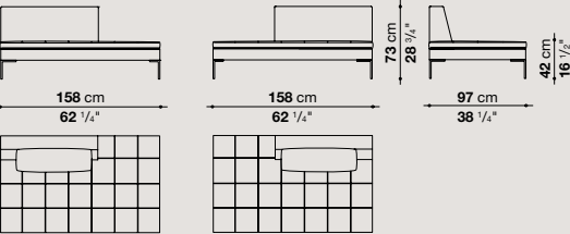
CH156TPS_Q / CH156TPD_Q
