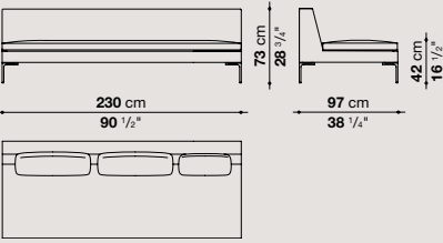
CH228C
