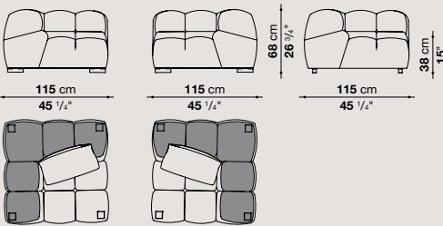
TY115_3S / TY115_3D
