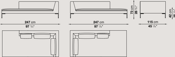
CHL247LS_1 / CHL247LD_1
