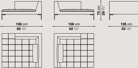
CHL135LS_Q / CHL135LD_Q
