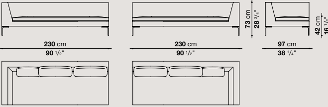
CH228S / CH228D
