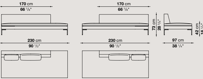
CH228TPS / CH228TPD
