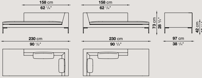
CH228LS / CH228LD
