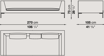
CHL270_1
