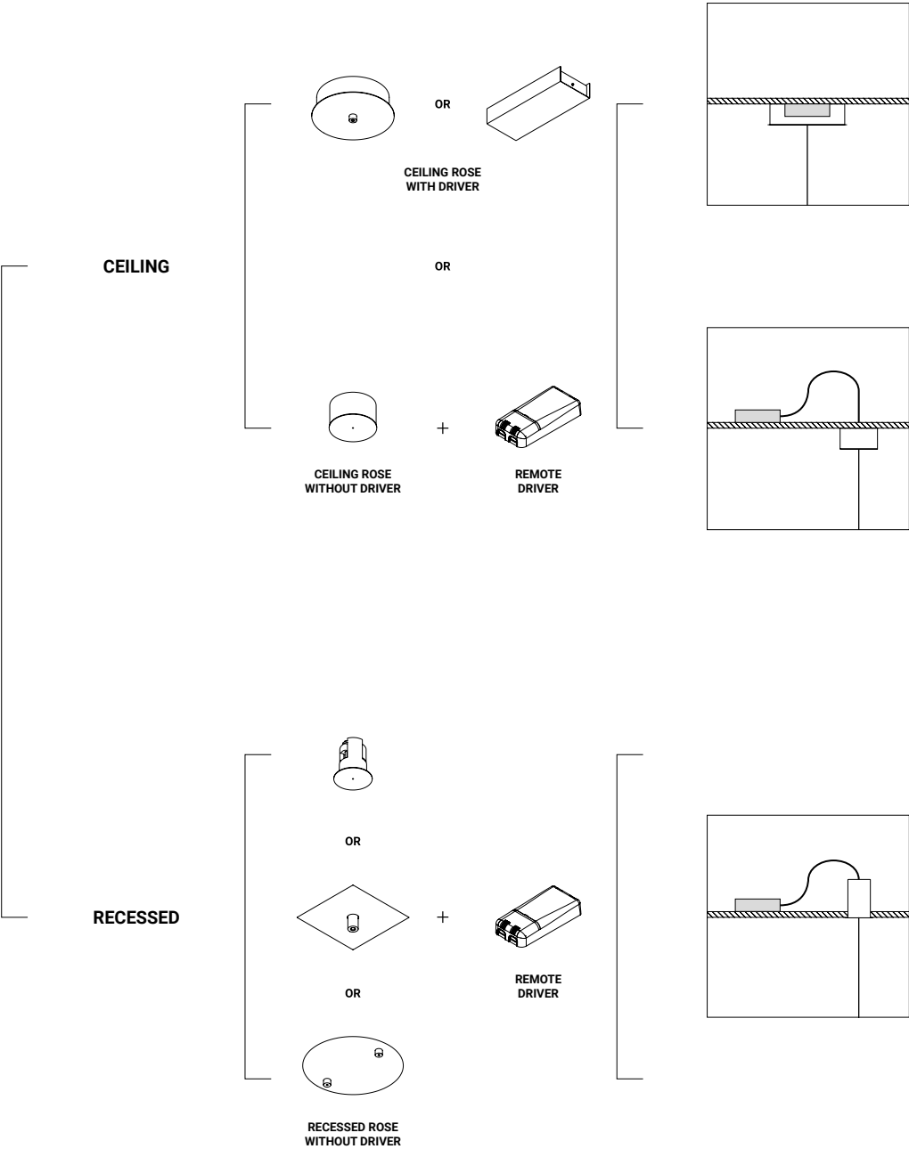
SUSPENSION LUMINAIRE code 1AXXXXXXX.XX.20
