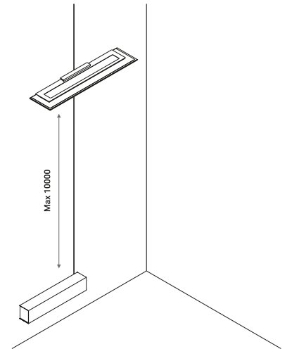
REFLEX: example of installation with wall/ceiling driver
