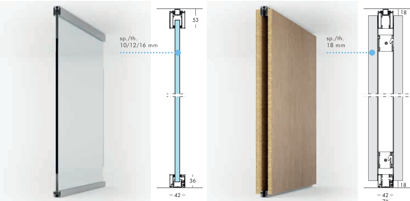
Parete divisoria vetrata Glazed partition wall Verglaste Wand Cloison vitrée Mampara acristalada
