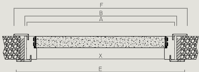
Quota pavimento finito Finished floor surface Sol fini Конечный пол
