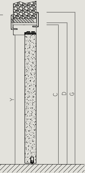
Quota pavimento finito Finished floor surface Sol fini Конечный пол
