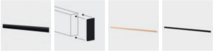
SKIRTING L Dark oak 2,5 x 19,8 (H) x 240 (L) cm END PIECE RECTANGULAR Black painted metal 2,5 x 6 (H) x 0,2 (L) cm RECTANGULAR SKIRTING Light oak 2,5 x 6 (H) x 240 (L) cm RECTANGULAR SKIRTING Dark oak 2,5 x 6 (H) x 240 (L) cm
